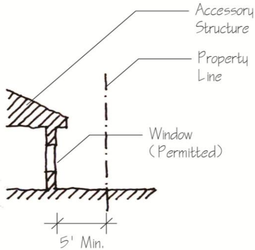
Section (Not to Scale)
