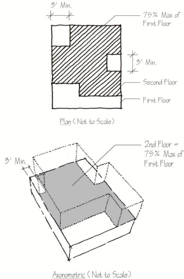
Figure WHWNOD-1 SECOND FLOOR AREA AS A PERCENT OF FIRST FLOOR
