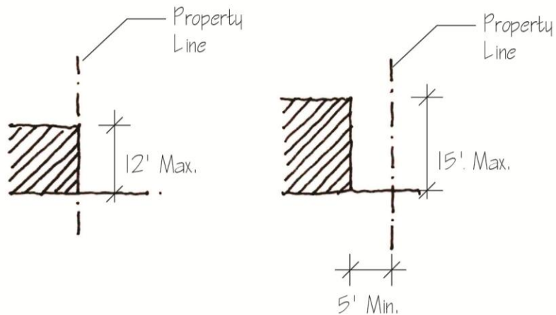
Figure WHWNOD-14 ACCESSORY STRUCTURE HEIGHT
